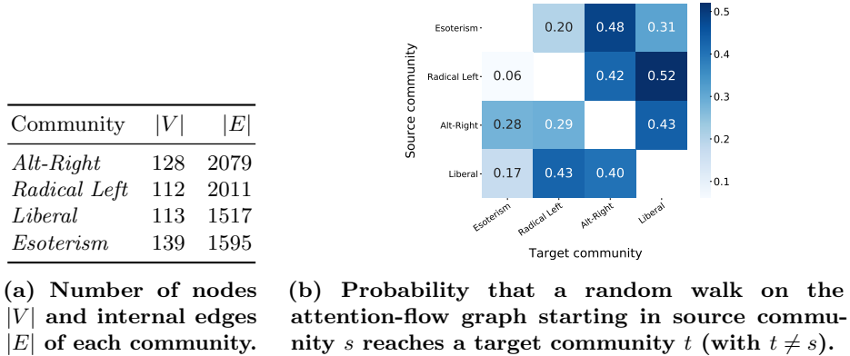
Fig. 2: Statistics on the four political communities considered.
